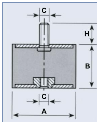
PLOTS CYLINDRIQUES 1 TIGE FILETEE 1 TARAUDAGE TYPE B
